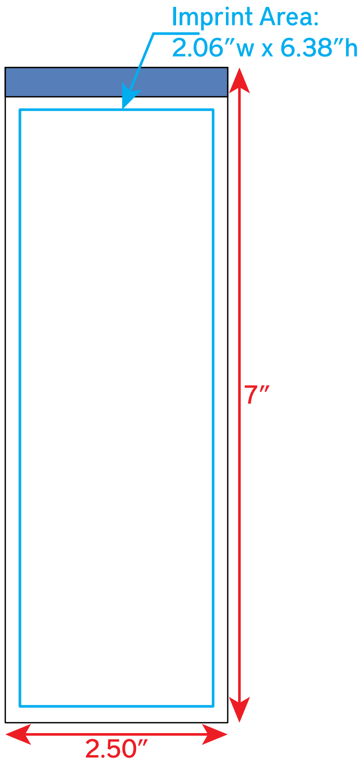
Front View
